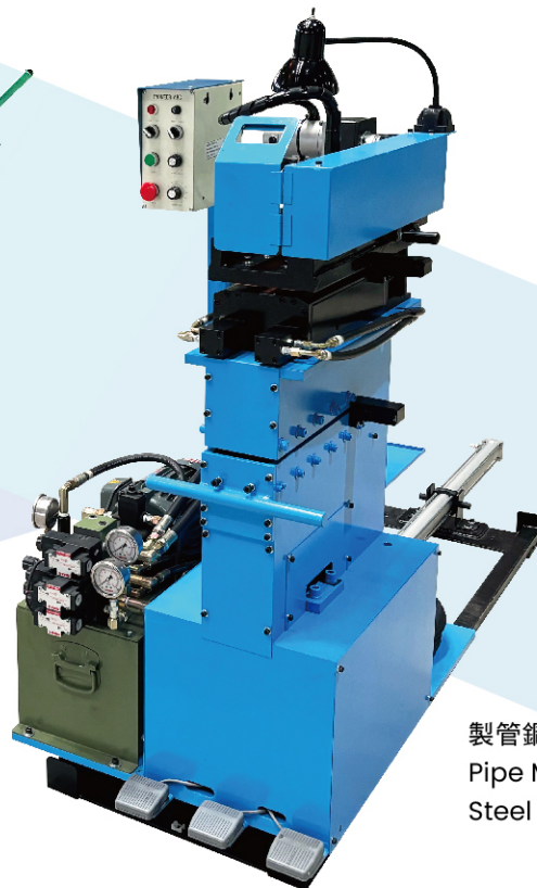
連續沖模業用裁鋸機 Industrial Continuous Stamping Shear Welder
