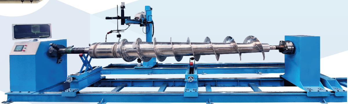
螺旋桿臥式自動銲接機 Horizontal Screw Rod Automatic Welding Machine
