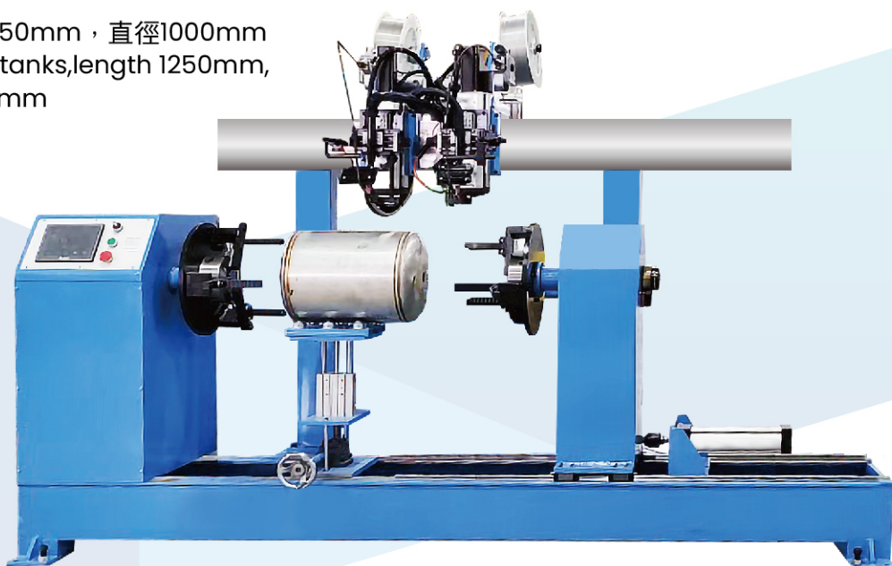
臥式雙槍銲接設備(送線添料系統) Horizontal Dual-Gun Welding Equipment (Wire Feeder)
