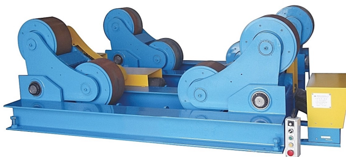
自調式滾輪 Self-Adjusting Roller
